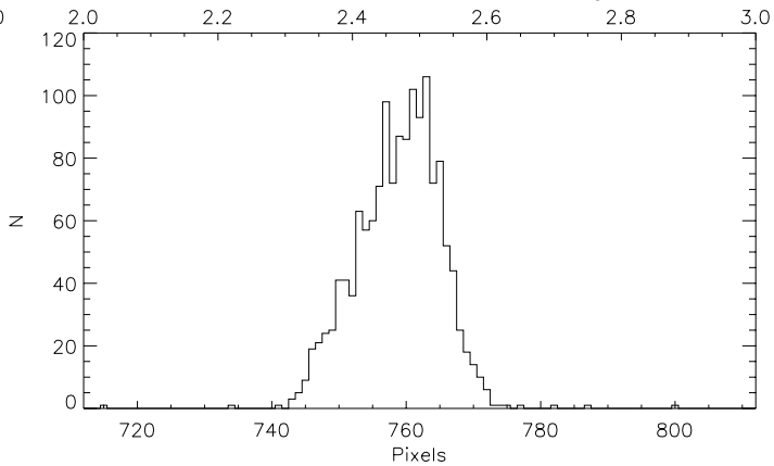
Cross-Dispersion Profile of FUV: Segment A
