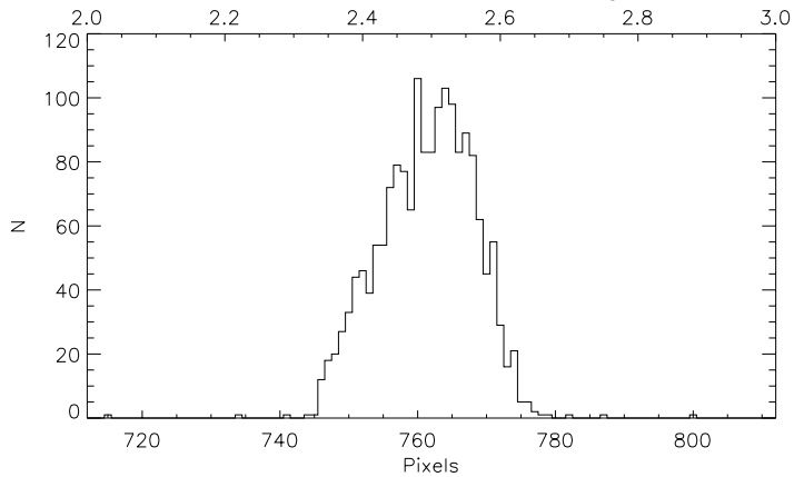
Cross-Dispersion Profile of FUV: Segment B
