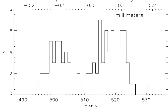
Cross-Dispersion Profile of FUV: Segment B
