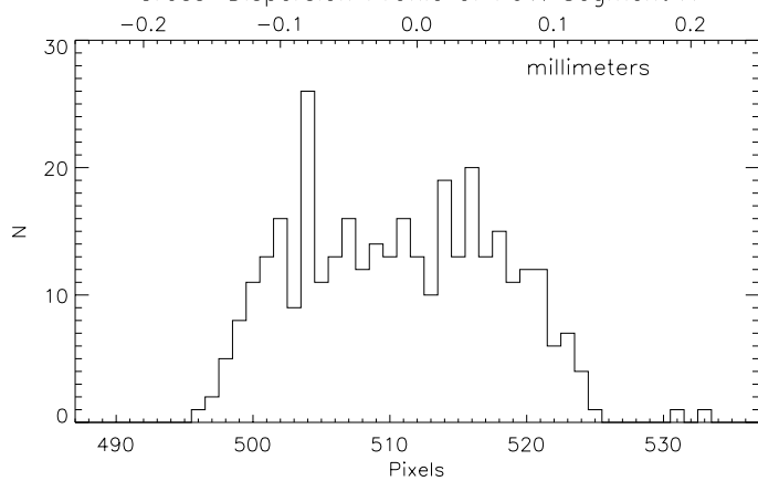
Cross-Dispersion Profile of FUV: Segment A
